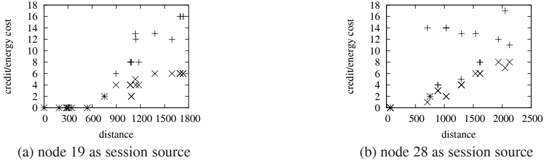
Figure 6: Relationship among Euclidean distance, payment, and forwarding energy cost. The points labeled with + are payment and those with x are forwarding energy cost.
