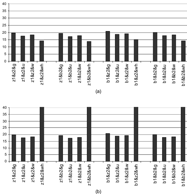
Fig. 4. The QoC metric of the data delivery chain: a) indoor; b) outdoor
